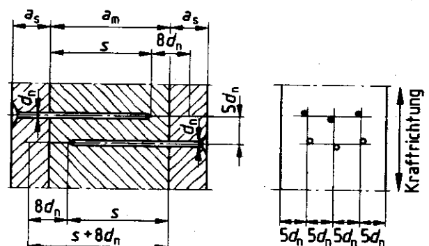
c) s < a_m < (s + 8 d_n)
